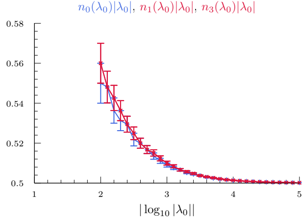
fig A6.1: plot of n_j(\lambda_0)|\lambda_0| for j = 0 (blue, color online) and j = 1, 3 (red) as a function of |\log_{10} |\lambda_0|| . This plot confirms (6.10).
