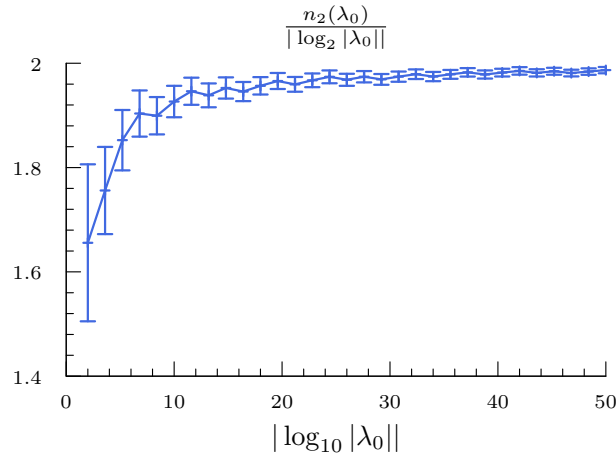
fig A6.2: plot of n_2(\lambda_0)|\log_2 |\lambda_0|^{-1} as a function of |\log_{10} |\lambda_0|| . This plot confirms (6.11).
