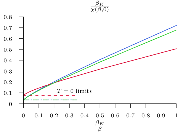
fig 6.6: plot of \frac{\beta_K}{\chi(\beta,0)} as a function of \frac{\beta_K}{\beta} for various values of \lambda_0 : \lambda_0 = -0.024 (blue), \lambda_0 = -0.02412 (green), \lambda_0 = -0.05 (red). In [Wi75], \lambda_0 = -0.024 and -0.02412 . Note that the abscissa of the data points are 2^{-n} for n \geq 0 , so that there are only 3 points in the range [0.25, 1] . The lines are drawn for visual aid.
