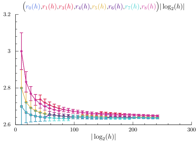
fig A6.3: plot of r_j(h)|\log_2(h)| as a function of |\log_2(h)| . This plot confirms (6.12).
