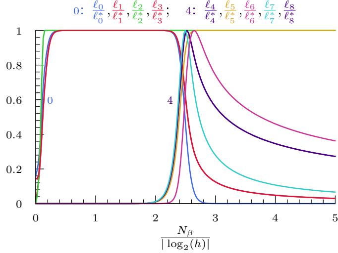
fig 6.4: plot of \frac{\ell_j}{\ell_j^*} as a function of the iteration step N_\beta for \lambda_0 = -0.125 and h = 2^{-40} . Here \ell_0^* through \ell_3^* are the components of the non-trivial fixed point \ell^* and \ell_4^* through \ell_8^* are the values reached by \ell_4 through \ell_8 of largest absolute value. The flow behaves similarly to that at h = 0 until \ell_4 through \ell_8 become large, at which point the couplings decay to 0, except for \ell_5 and \ell_2 .
